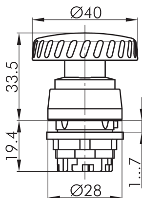
Dimensional drawing
