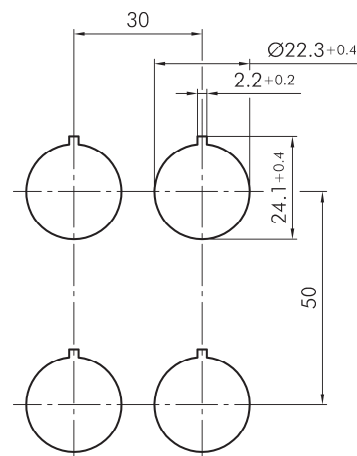
Drilling pattern
