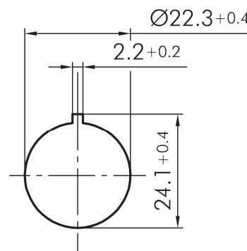
Drilling pattern
