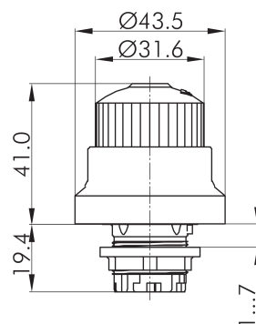
Dimensional drawing
