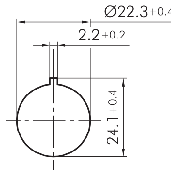
Drilling pattern
